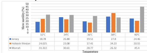
Fig. 4. Effect of temperature on spermatozoa slow progressive motility of different breed
